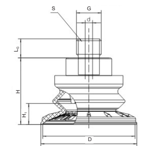
Installation method of external thread M
