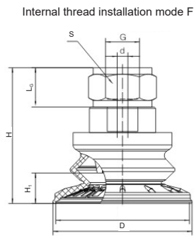
Internal thread installation mode F
